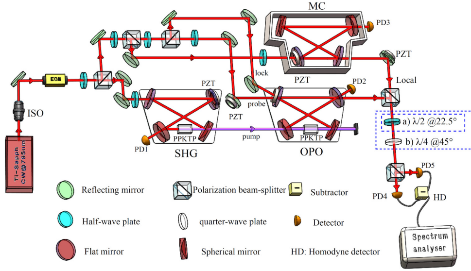
Fig. 2. Schematic of experimental setup. Optics in (a) and (b) are included to measure the variance of \hat{S}_2 and \hat{S}_3 , respectively. Removing the (a) and (b), the variance of \hat{S}_0 and \hat{S}_1 is measured when the two outputs of photocurrents are added and subtracted.
