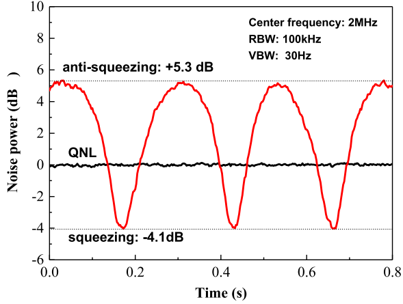
Fig. 3. Measured noise power of \hat{S}_2 , as relative phase between the generated amplitude squeezed light and the bright coherent light is scanned. The analyzing frequency is 2 MHz in the zero-span mode with RBW = 100 kHz, and VBW = 30 Hz.
