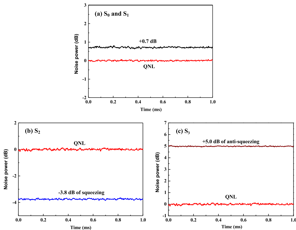
Fig. 4. Quantum noises of Stokes operators of polarization squeezed beam. (a) \hat{S}_0 and \hat{S}_1 ; (b) \hat{S}_2 ; (c) \hat{S}_3 . The measurements are taken at 2 MHz in the zero span mode with RBW = 100 kHz and VBW = 30 Hz. The data is averaged for 20 times.
